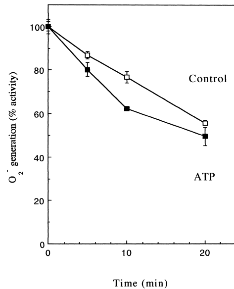
Fig. 6. Effect of ATP on the stability of NADPH oxidase activated in a semi-recombinant system. The semi-recombinant activation mixture was diluted 25-fold with 10 mM PIPES (pH 7.0) or the buffer containing 1 mM ATP and incubated at 0°C for a given time. An aliquot of the mixture was taken up and assayed for O 2 - generation. The results are expressed as means \pm S.D. of three determinations. The initial activity of the diluted sample with or without ATP was 304 \pm 11.2 or 420 \pm 4.3 nmol/min/mg, respectively.
