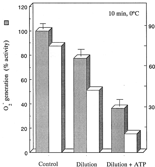
Fig. 5. Effect of ATP on NADPH oxidase activity and F-actin content. After activation with SDS, the cell-free mixture was diluted 25-fold with 10 mM PIPES buffer (pH 7.0) with or without 1 mM ATP, and incubated at 0°C for 10 min. The mixture was then assayed for O 2 - generation, and the activities are expressed as means \pm S.D. of three determinations. The activity without incubation is taken as 100% activity (1210 \pm 67 nmol/min/mg). F-actin estimation was performed as described in Section 2. This is a typical result of two independent experiments.
