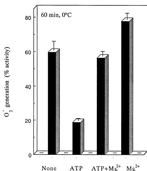
Fig. 3. Prevention of ATP-induced deactivation of NADPH oxidase by Mg^{2+} . The cell-free mixture was diluted and incubated for 60 min at 0°C in the presence and absence of 1 mM ATP and/or 8 mM MgCl_2 . The mixture was assayed for O_2^- generation. The activity without incubation is taken as 100% activity ( 1204 \pm 57 nmol/min/mg). Data are expressed as means \pm S.D. of three determinations.
